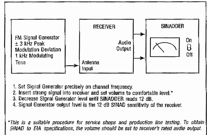
Figure 2. SINAD measurement using the SINADDER™
