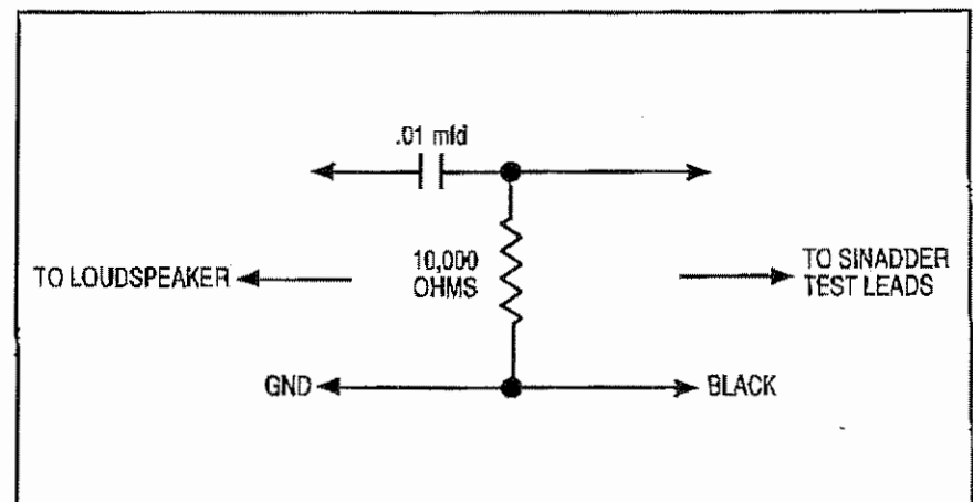
Figure 3. Auxiliary Filter Circuit
