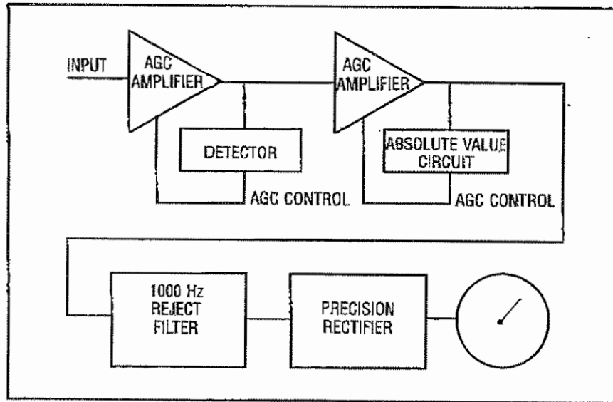
Figure 1. SINADDER™ Block Diagram
